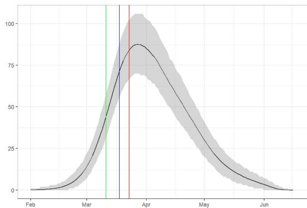
Figure 2. SIR model simulations calibrated to an incidence of 150 cases/day on 01/09/20 and 700 cases/day on 01/10/20 (for details see Appendix 2). Key inputs are the delay until interventions are introduced that are effective in reversing the growth in incidence and the post-intervention R value. Key outputs are the absolute number of infections acquired post-01/10/20 (B) and the fraction of all infections these represent (B/A). Scenarios range from optimistic (current interventions are
