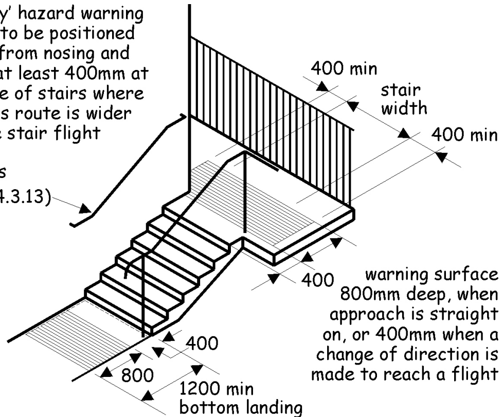
Figure 4.6 Use of corduroy tactile paving
